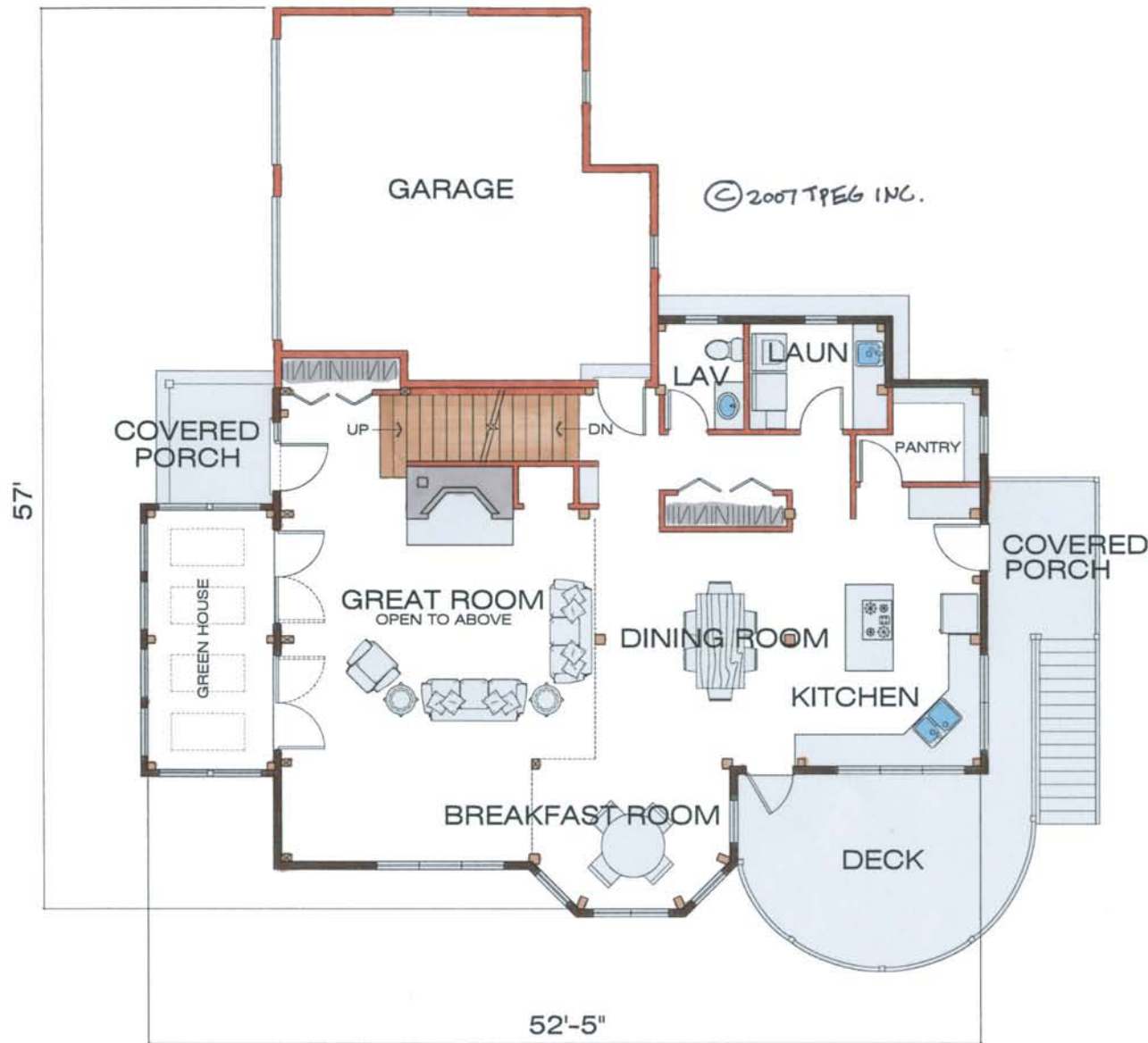
FIRST FLOOR PLAN 1442 SQ. FEET
