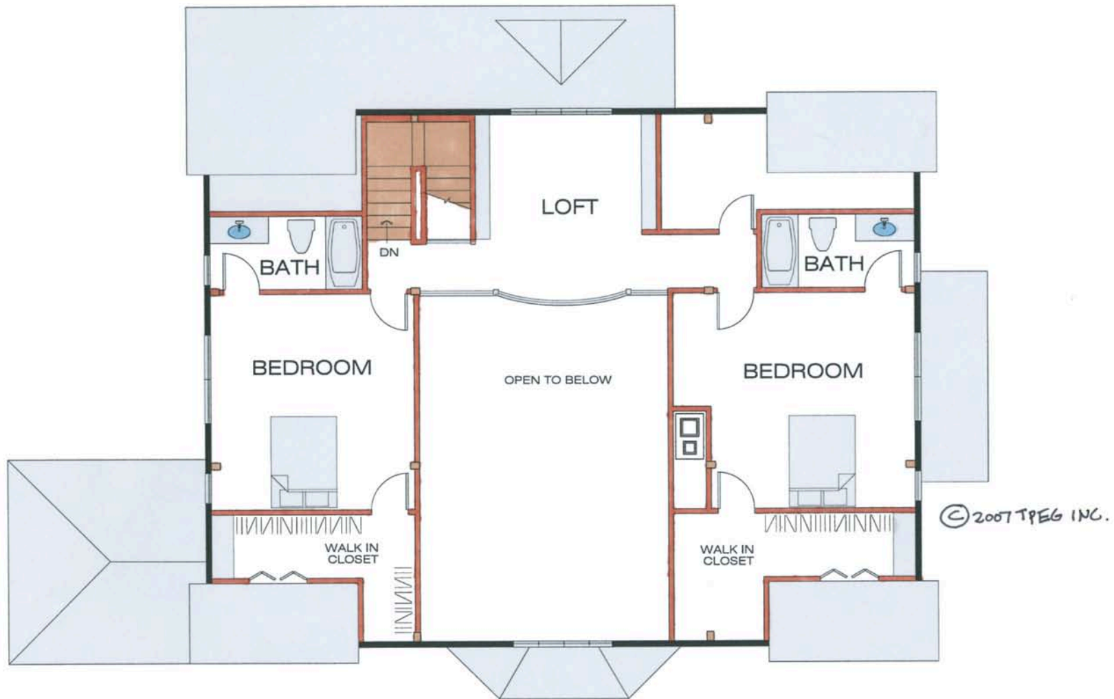
SECOND FLOOR PLAN 1164 SQ. FEET
