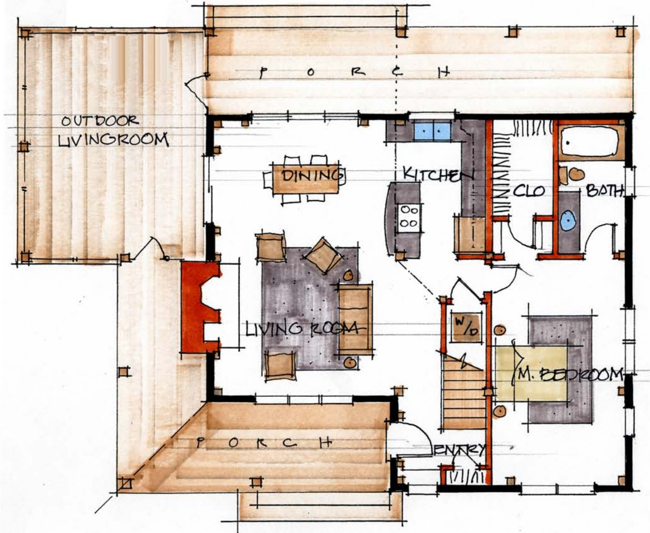
FIRST FLOOR 1029 SQ. FEET
