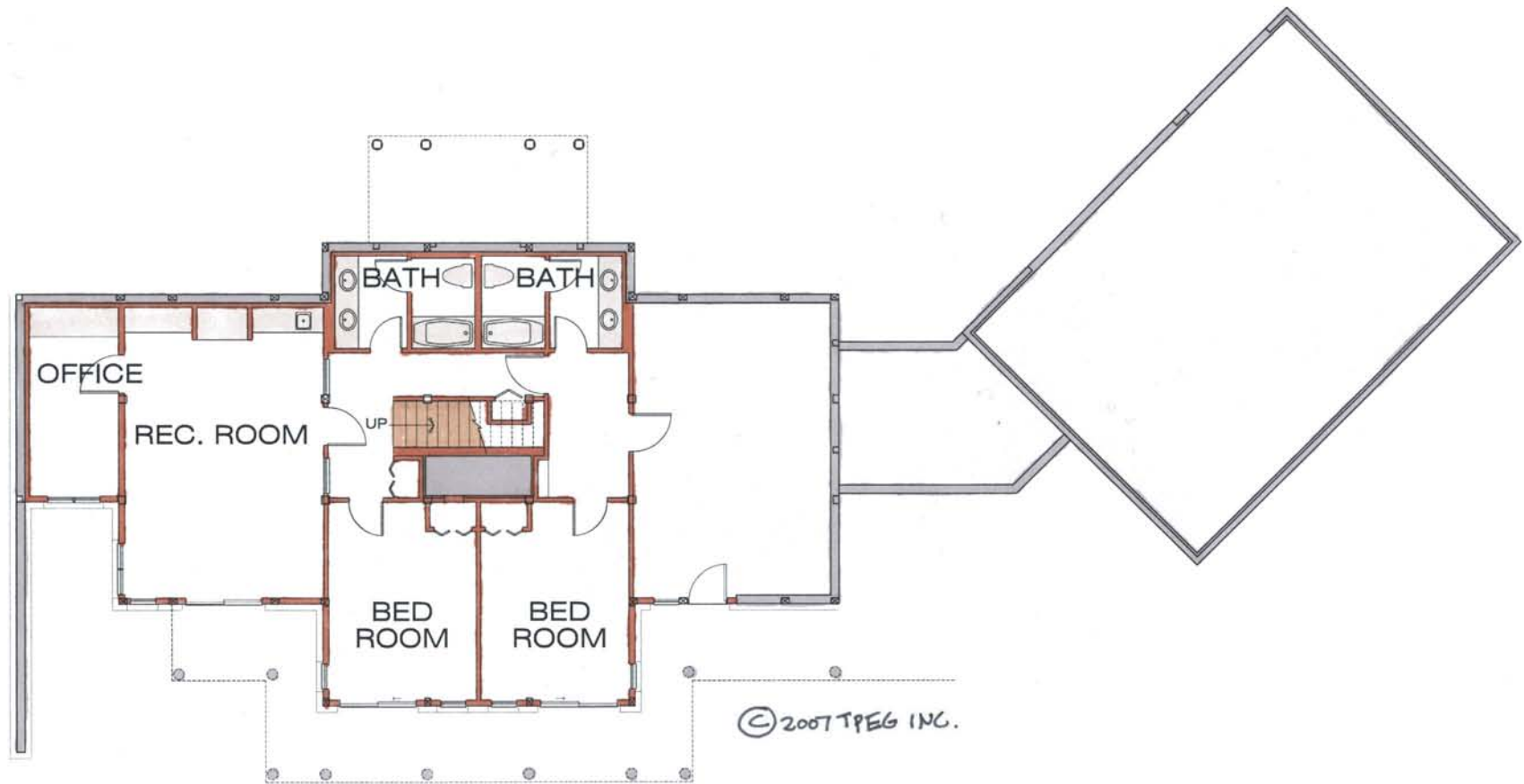
BASEMENT PLAN 1600 SQ. FEET
