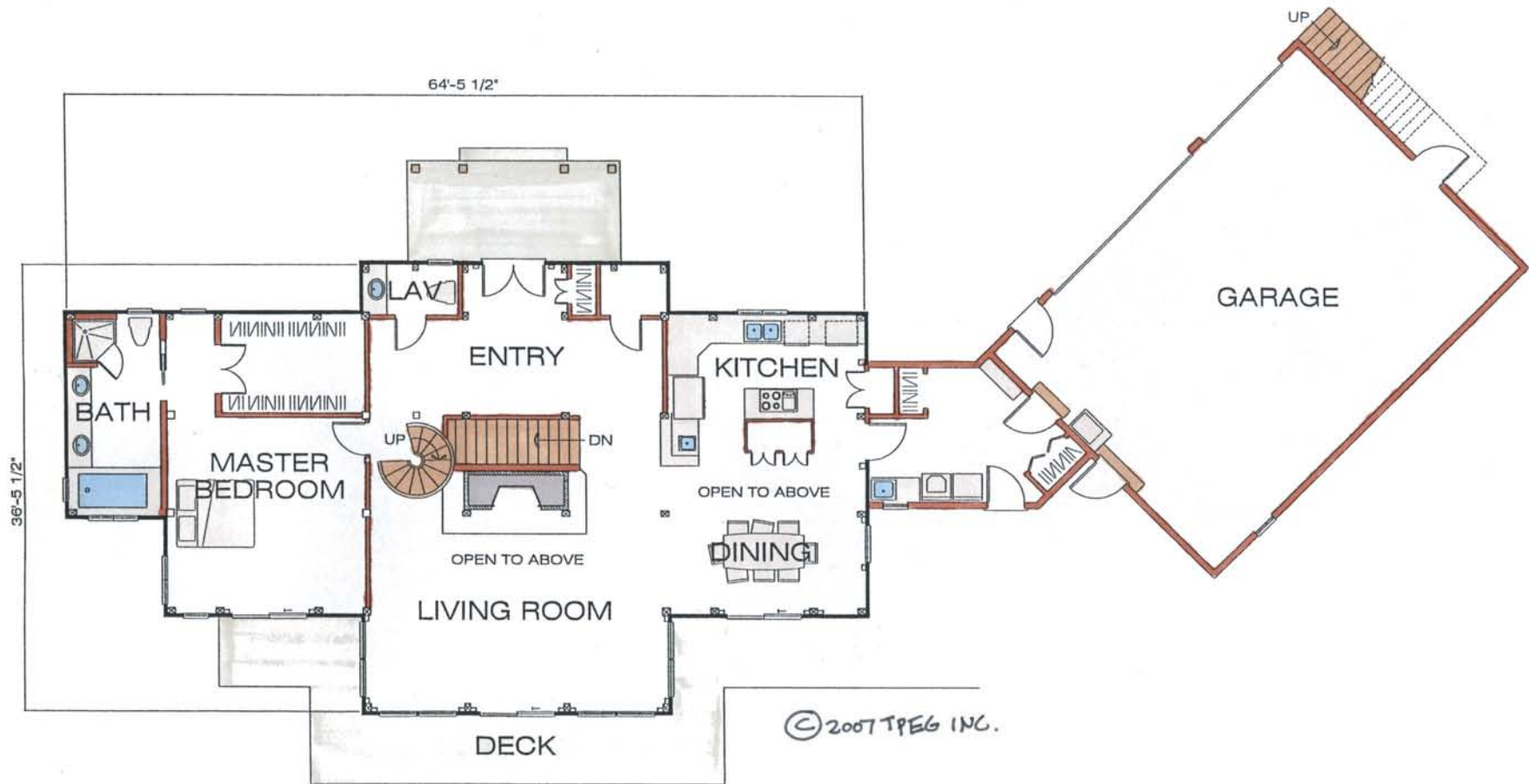
FIRST FLOOR PLAN 1800 SQ. FEET
