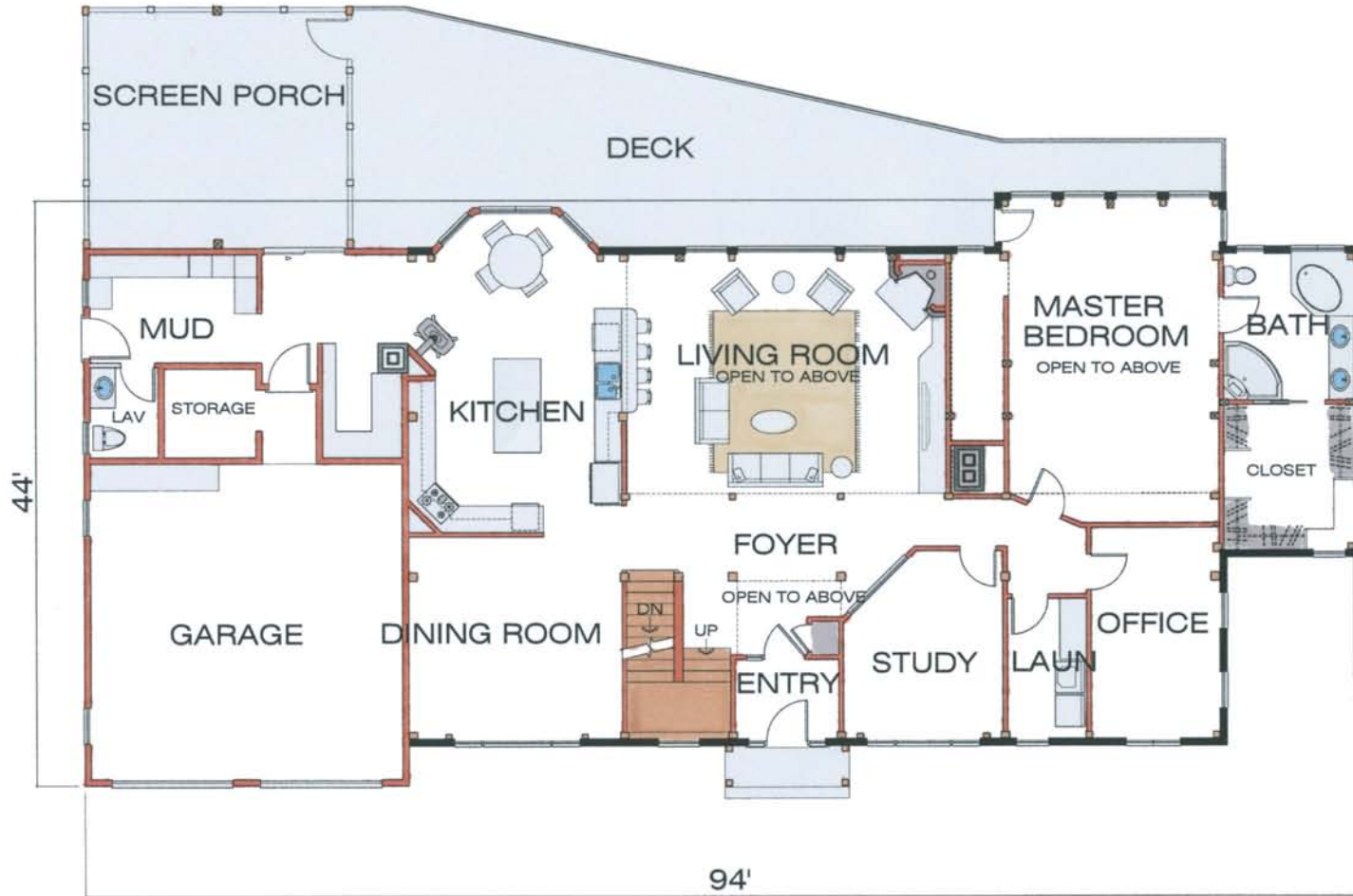
FIRST FLOOR PLAN 2826 SQ. FEET
