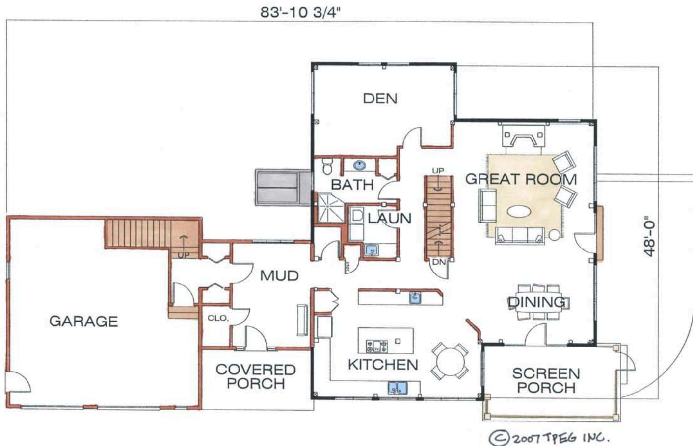
FIRST FLOOR PLAN 1870 SQ. FEET
