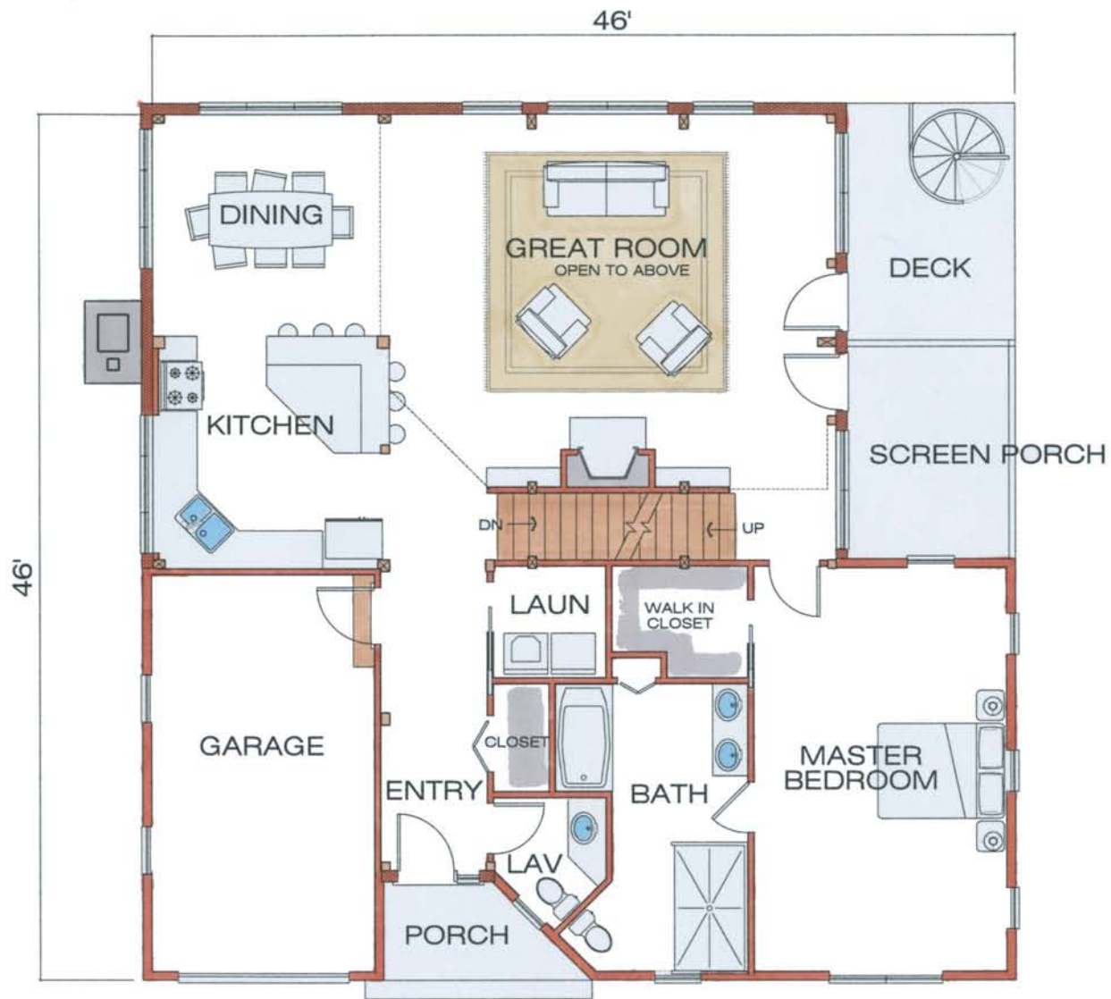
FIRST FLOOR PLAN 1521 SQ. FEET
